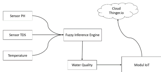
FIGURE 5. FUZZY DESIGN
