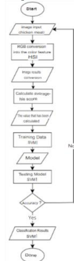
FIGURE 2. Classification Flowchart SVM
