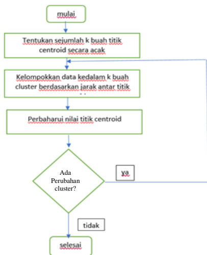
Fig. 4. Flowchar kerja algoritma K-means (peneliti,2021)
