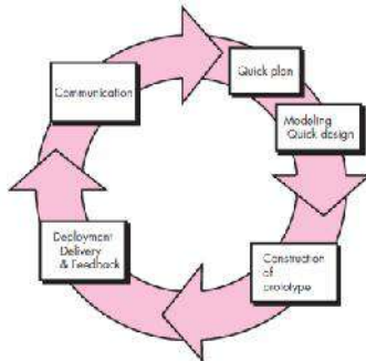
Gambar 1. Metode Prototype
