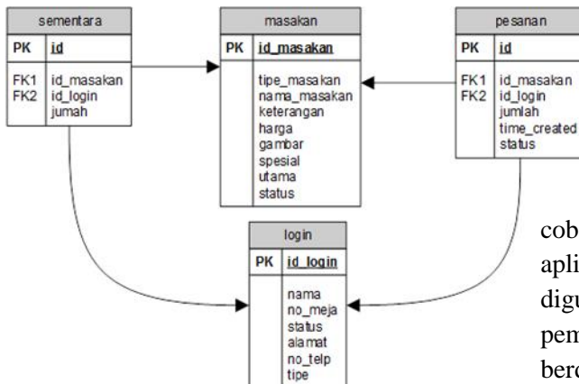
Gambar 10 : Relasi Database Diagram
