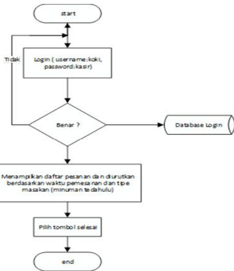
Gambar 6 : Flowchart Program Koki
