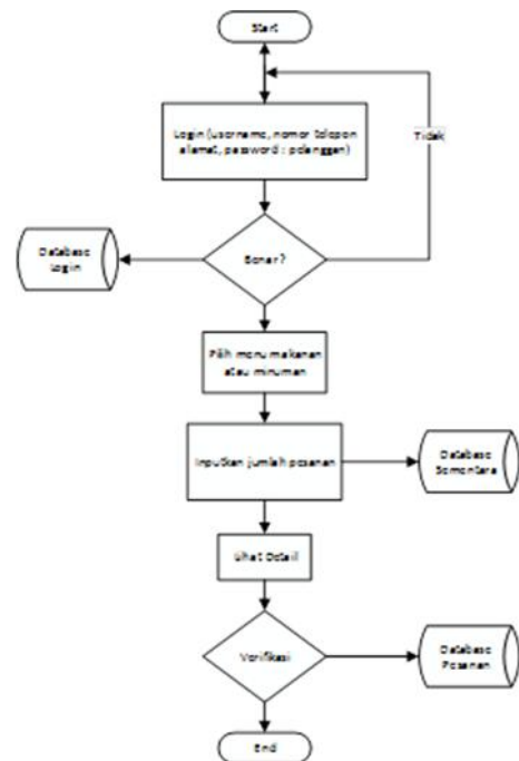
Gambar 5 : Flowchart Program Pesan – Antar
