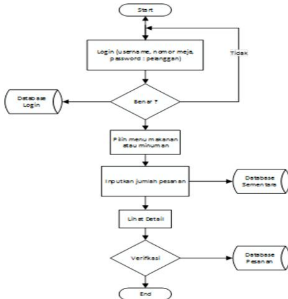
Gambar 4 : Flowchart Program Pelanggan
