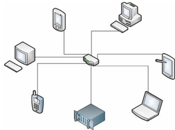
Gambar 2 : Client-Server
